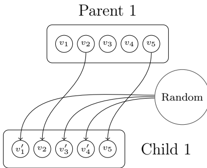
FIGURE 6.5 – Random based mutation operator
