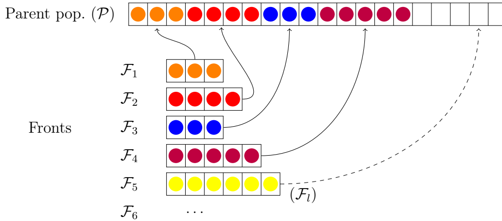
FIGURE 6.6 – NSGA-II and NSGA-III parent selection
