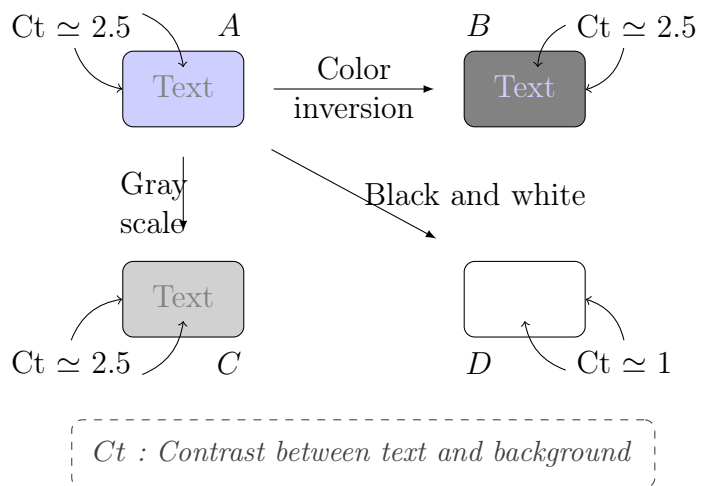
FIGURE 4.8 – Filter application
