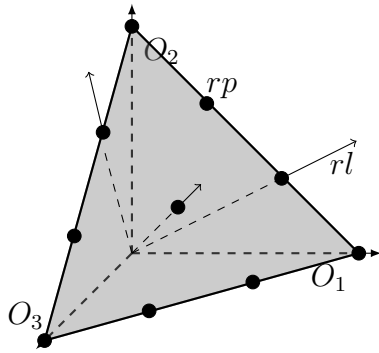
FIGURE 6.2 – NSGA-III hyperplane and reference points and lines
