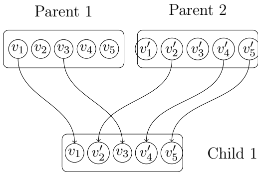
FIGURE 6.3 – Single child crossover operator
